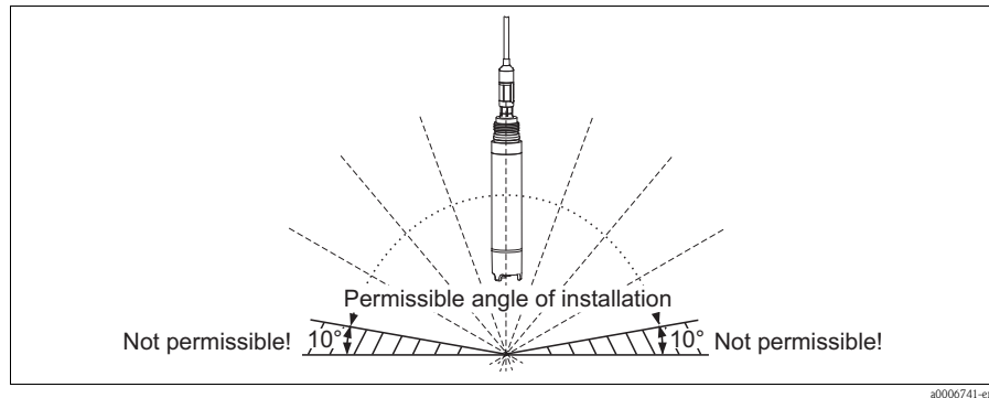
Fig. 2: Permissible angle of installation
