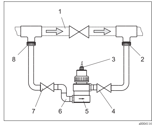
Fig. 10: Bypass installation with manually actuated valves or solenoid valves
