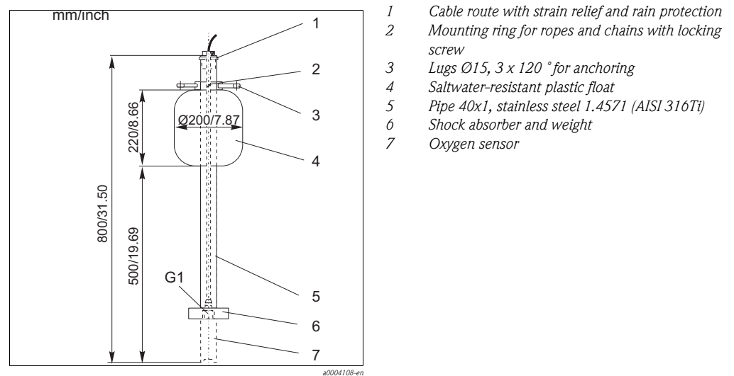
Fig. 8: Floating body
