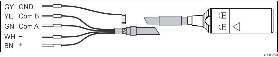
Fig. 13: Measuring cable CYK10
