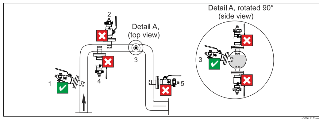
Fig. 11: Permissible and impermissible sensor installation positions
