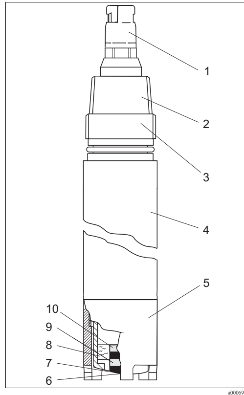
Fig. 14: Sensor design
