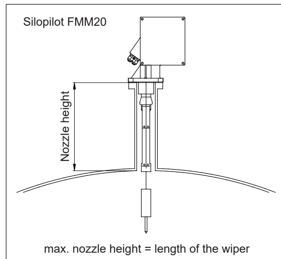
Mounting with wiper extensions
