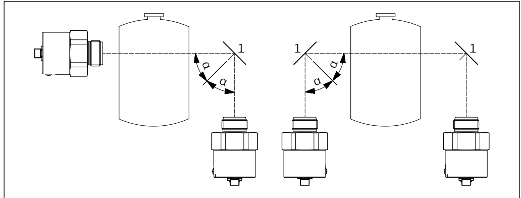
7 Reflector operation
