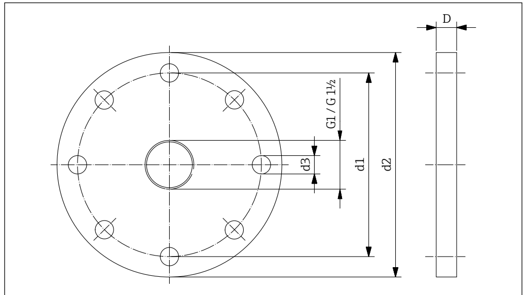
32 Dimensions mounting flange (Connection dimensions according to DIN EN 1092-1)
