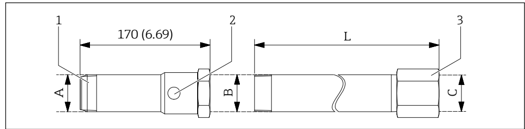
40 Dimensions high temperature adapter with extension. Unit of measurement mm (in)
