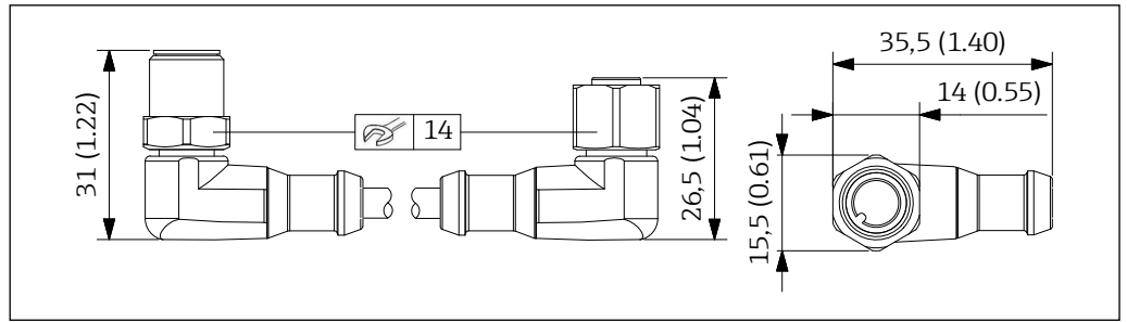
000000135 27 Connecting cable with M12 right-angle plug and M12 right-angle socket. Unit of measurement mm (in)
