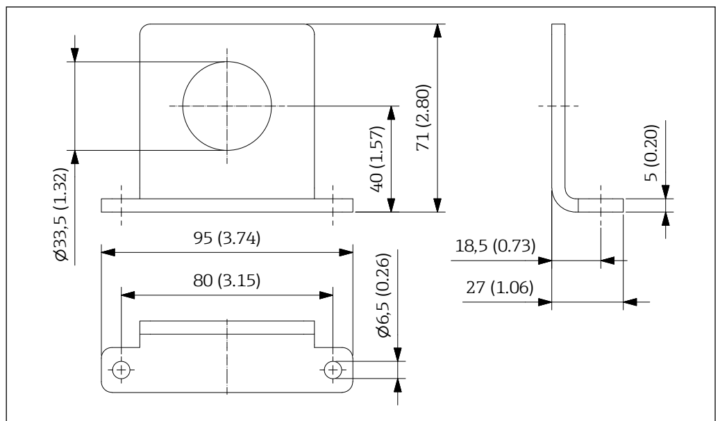
000000037 29 Dimensions mounting bracket. Unit of measurement mm (in)
