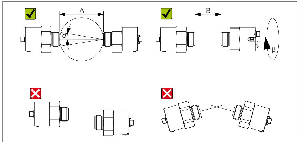
5 Mounting position
