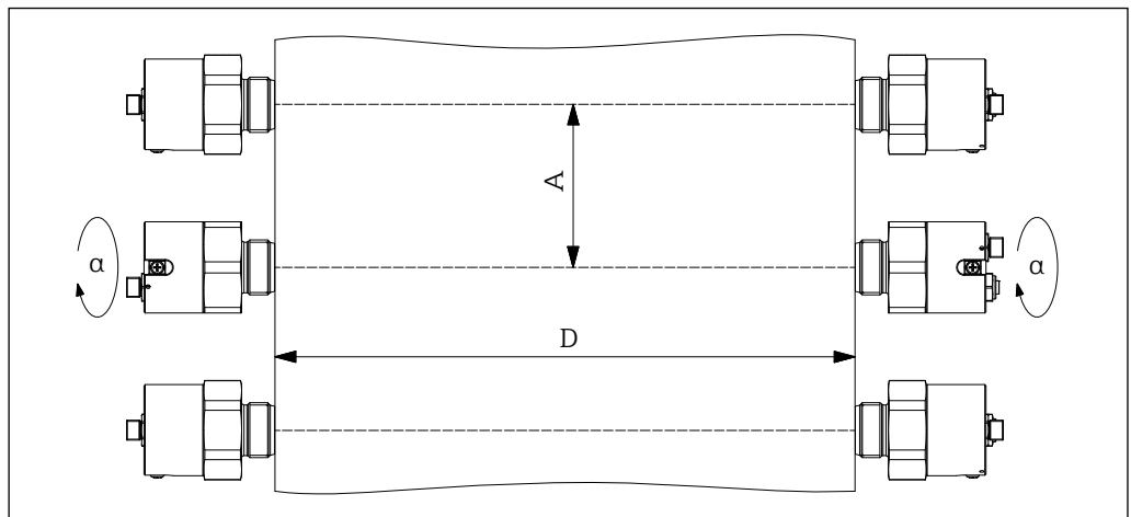
8 Parallel operation
