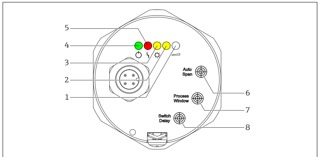
23 Display and operating elements of the FDR16
