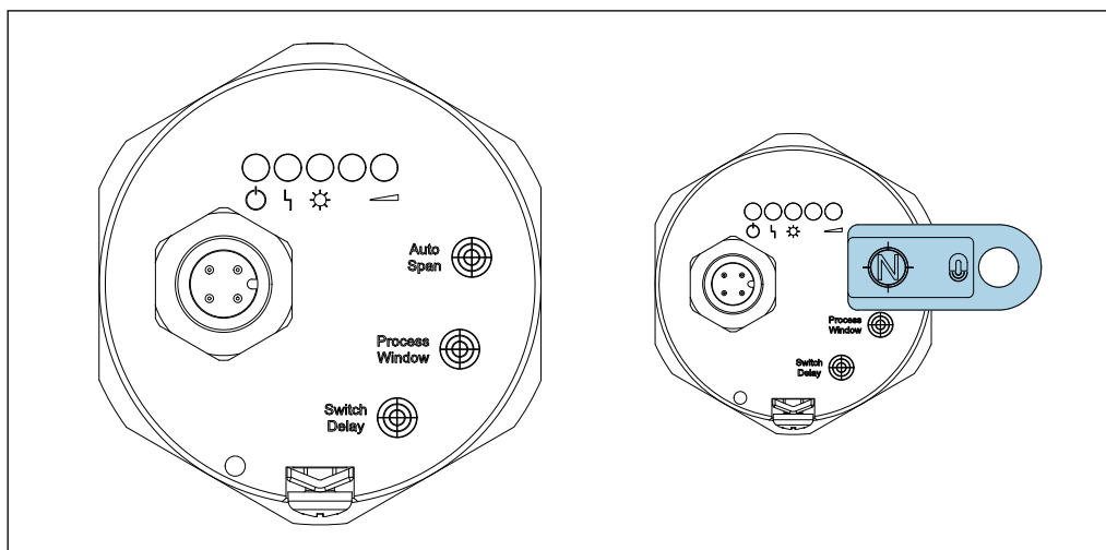
24 On-site operation
